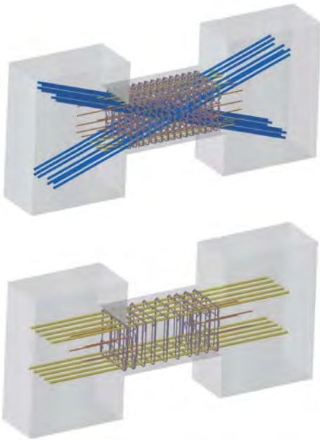
Figure 9. Diagonally reinforced coupling beam (top) and SFRC coupling beam (bottom).
