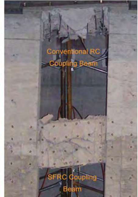
Figure 10. Coupling beam testing at the University of Michigan. © Rémy D. Lequesne.
