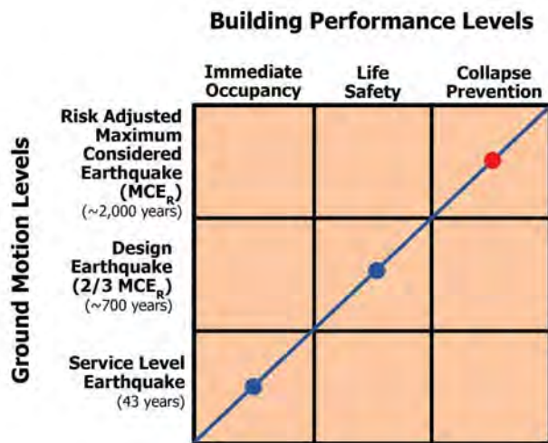
Figure 5. Seismic building performance matrix.
