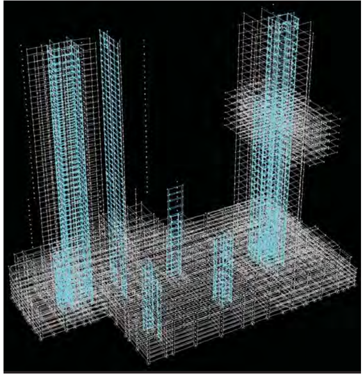
Figure 8. Nonlinear analysis model.
