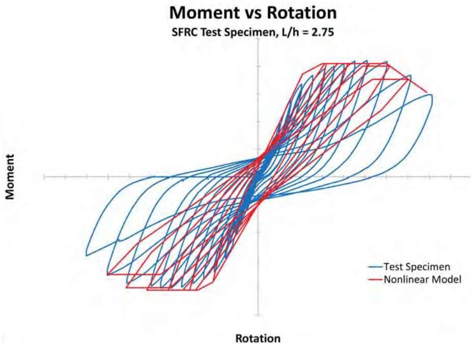
Figure 11. SFRC hysteresis loop.
