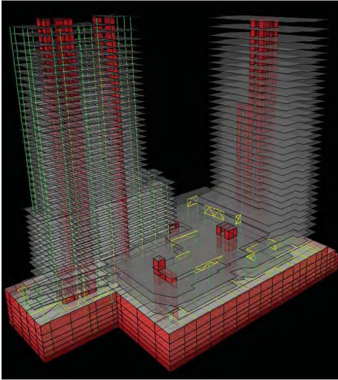
Figure 7. Linear analysis model.
