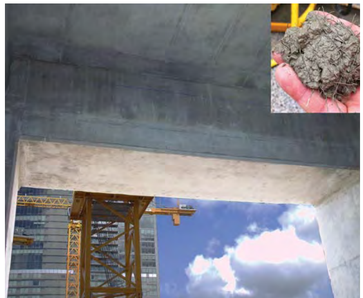
Figure 4. Steel-fiber reinforced concrete (SFRC) coupling beams.
